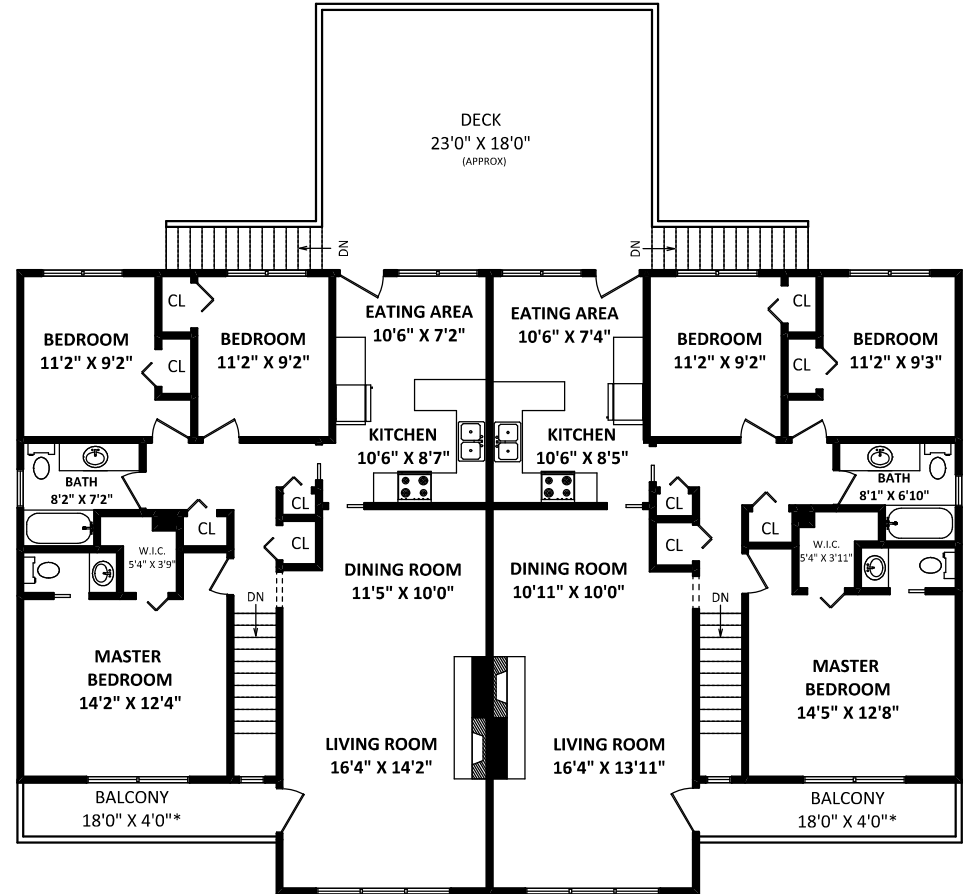
5437 FINISHED MAIN FLOOR: 1282 SQ.FT.
