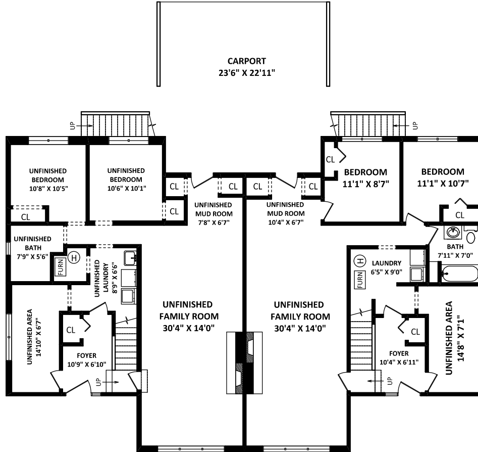
5437 TOTAL LOWER FLOOR: 1227 SQ.FT. FINISHED AREA: 122 SQ.FT. UNFINISHED AREA(S): 1105 SQ.FT.
